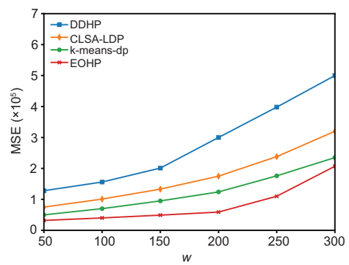
Fig. 7 Mean squared error (MSE) analysis of window size w on data utility based on the UK Car Accident Dataset
