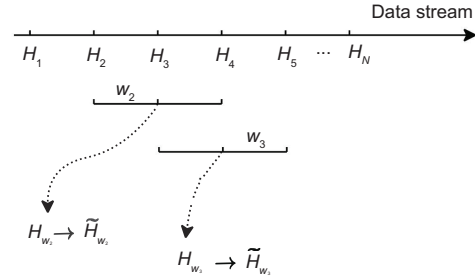
Fig. 1 Histogram publishing process using the sliding window model
